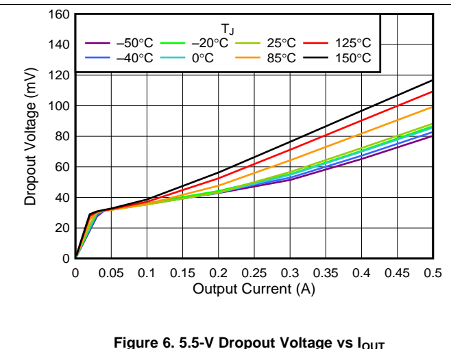
Figure 6. 5.5-V Dropout Voltage vs I_{OUT}
