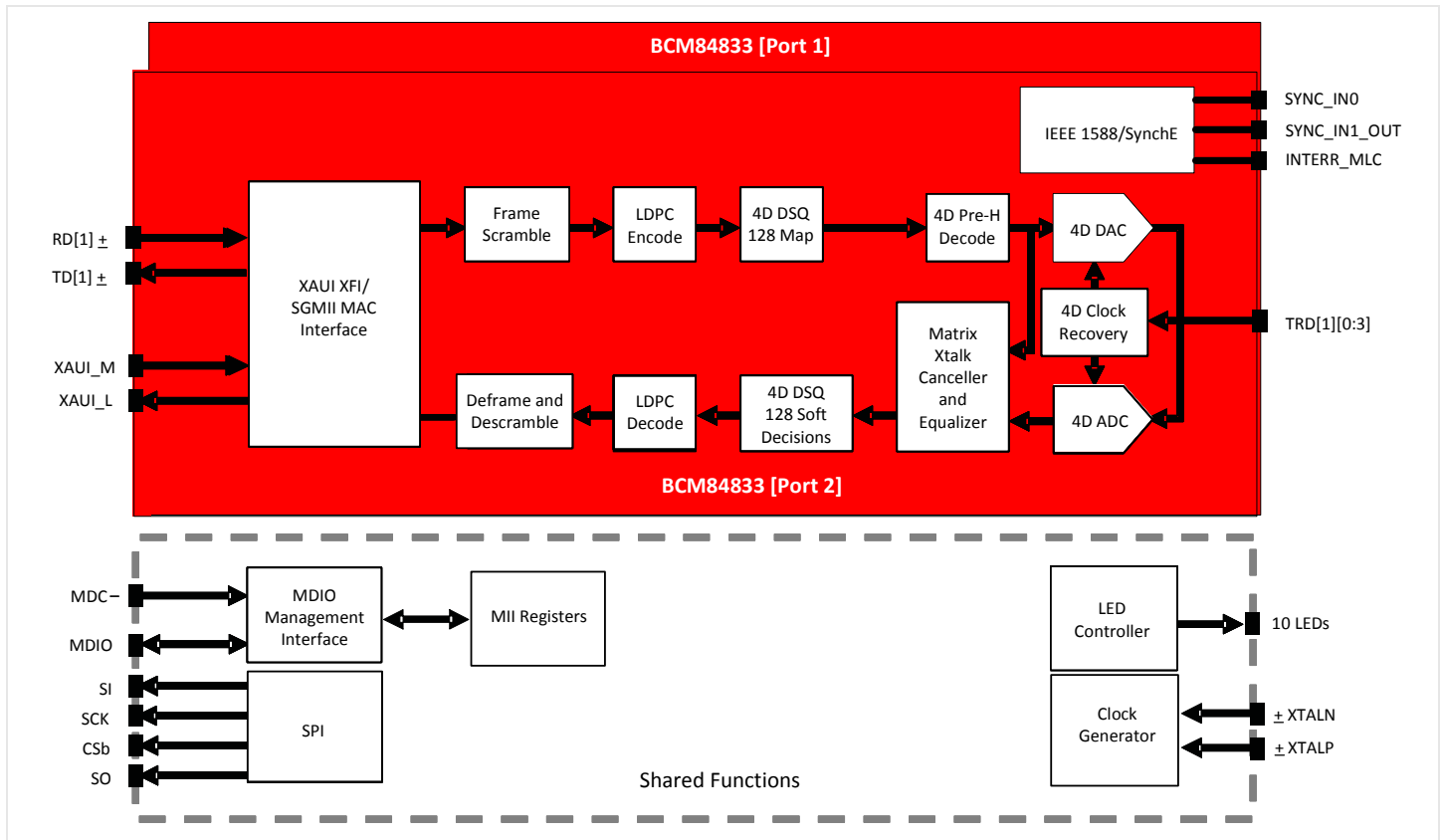
BCM84833 Block Diagram for Each Port
