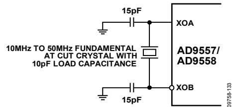
Figure 33. System Clock Input (XOA, XOB) in Crystal Mode (Recommended C_{LOAD} = 10\text{ pF} is Shown; Values of 15 pF Shunt Capacitors Shown Here Must Equal 2 \times (C_{LOAD} - C_{STRAY}) , Where C_{STRAY} is Typically 2 pF to 5 pF)
