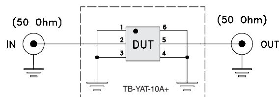
Fig 1. Block diagram of Test Circuit used for characterization, Test board TB-YAT-10A+ Conditions: Attenuation, VSWR: Pin=-10 dBm
