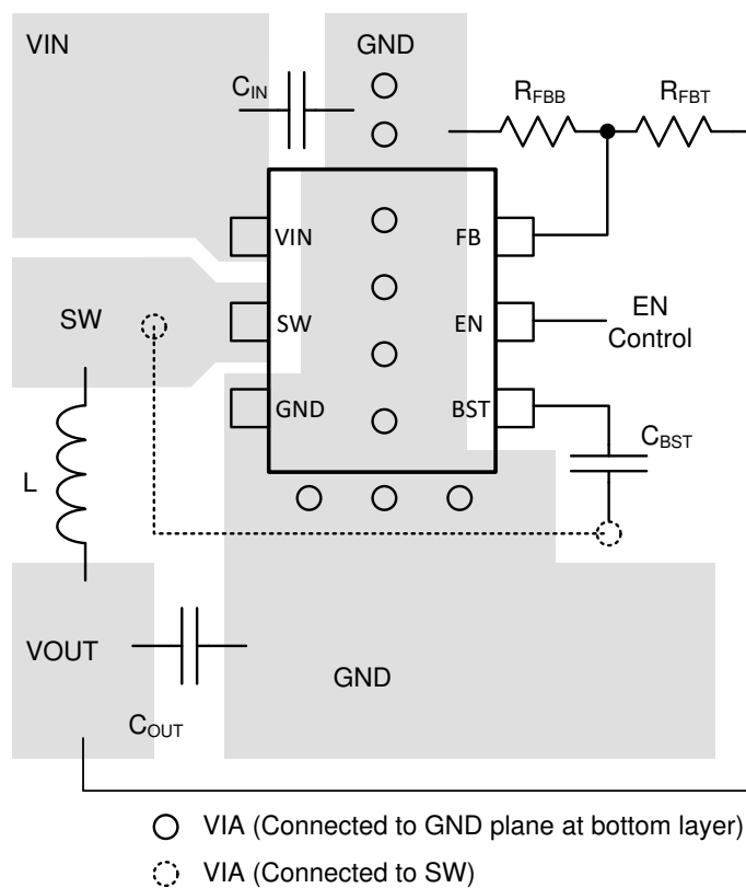
Figure 11-1. TPS563207S Layout
