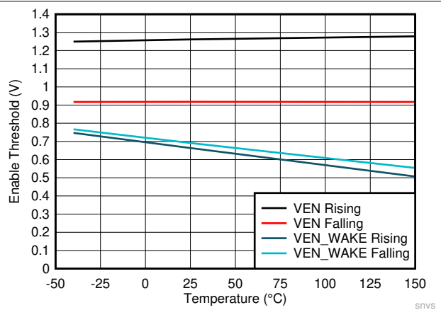
Figure 7-6. Enable Thresholds
