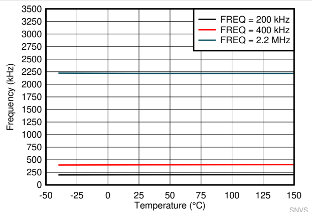
Figure 7-4. Switching Frequency
