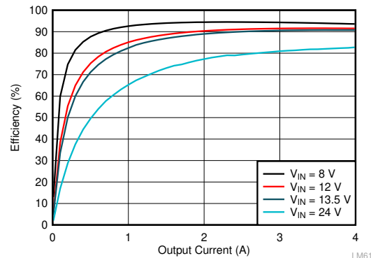
Figure 9-6. LMQ62440-Q1 Efficiency
