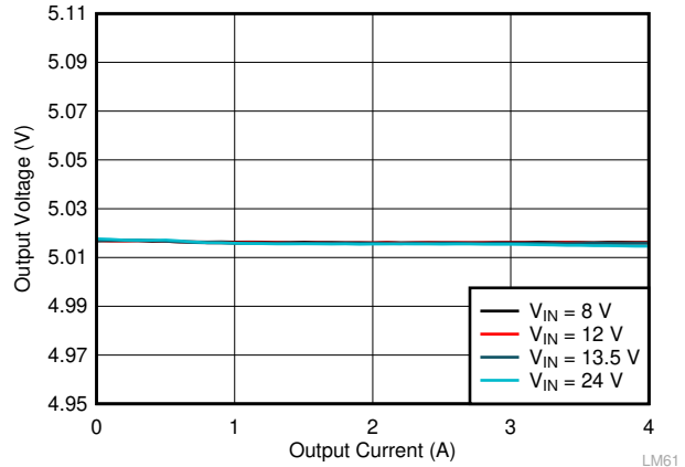
Figure 9-12. LMQ62440-Q1 Load and Line Regulation
