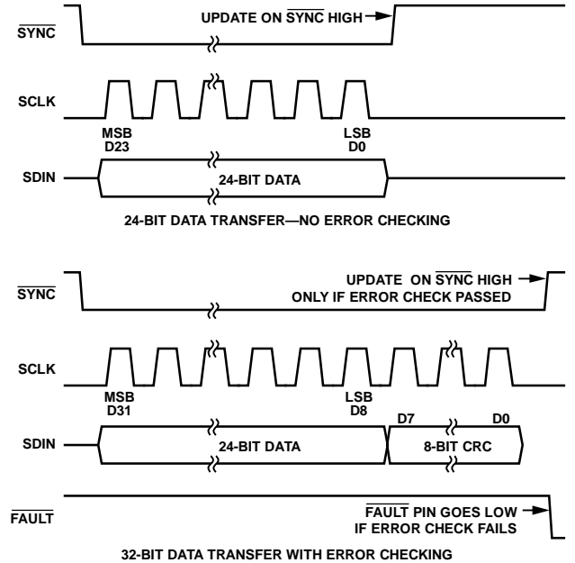
Figure 78. PEC Timing
