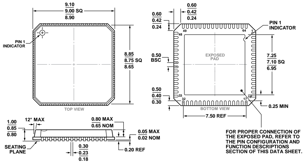
Figure 88. 64-Lead Lead Frame Chip Scale Package [LFCSQ_VQ] 9 mm × 9 mm Body, Very Thin Quad (CP-64-3) Dimensions shown in millimeters
