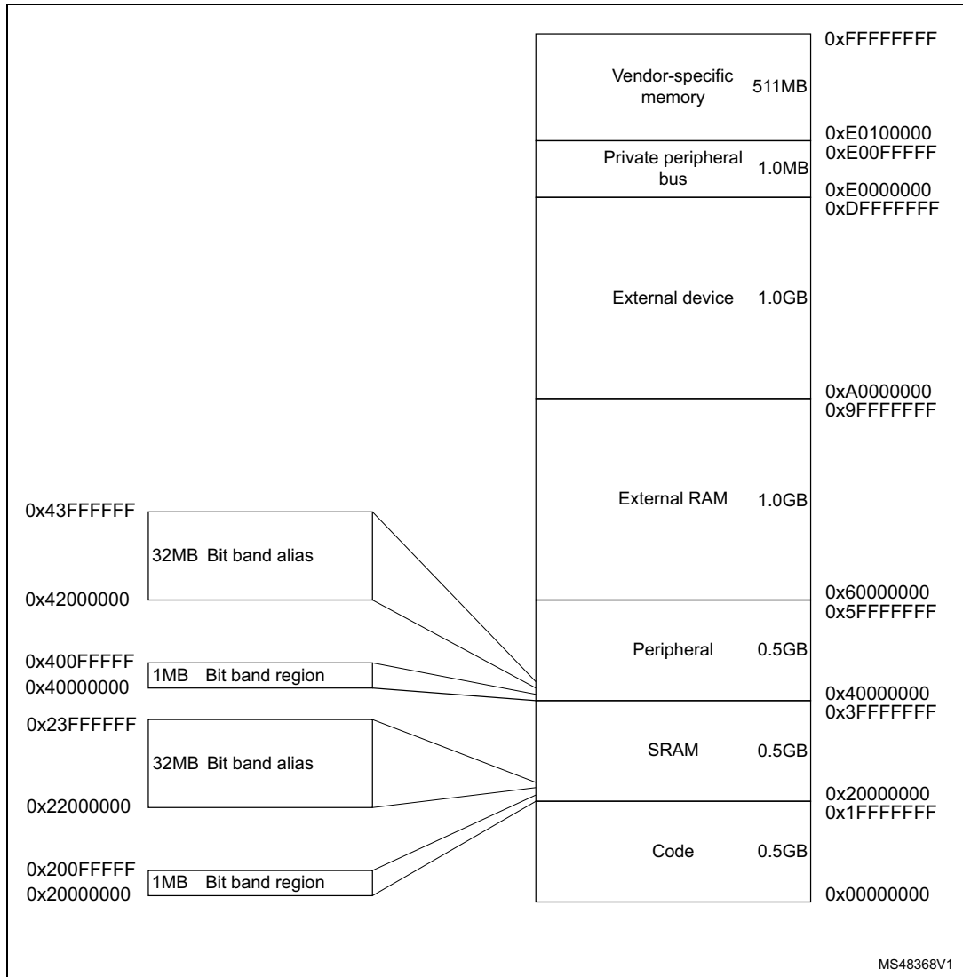
Figure 9. Memory map
