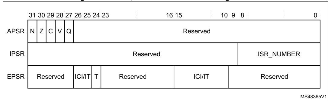
Figure 4. PSR bit assignments
