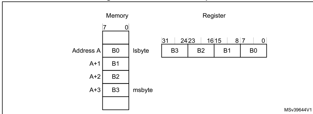
Figure 11. Little-endian example
