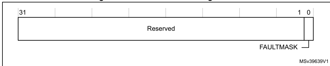
Figure 6. FAULTMASK bit assignments
