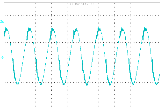
Output voltage ripple at nominal input voltage and max load current (20mV/div, 2us/div) Load cap: 10µF, tantalum capacitor and 1µF ceramic capacitor. Bandwidth: 20MHz.
