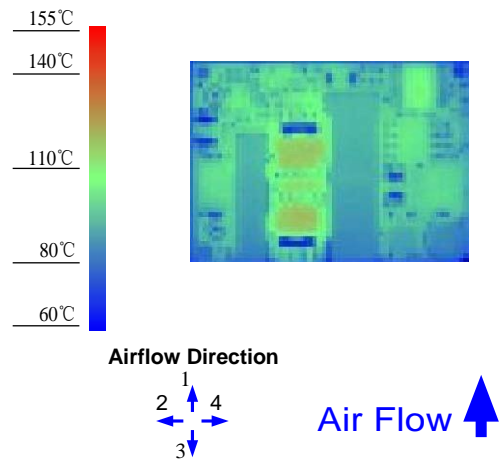
Figure 8. Thermal Image for Airflow Direction 1 (29A output, 55°C ambient, 200LFM, typical Vin, open frame, unit soldered onto a fixture board.)
