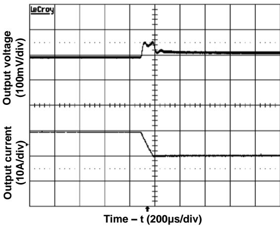
Figure 5. Transient Load Response (Typical Vin, 75% to 50% full load step at a slew rate 0.1A/µs)
