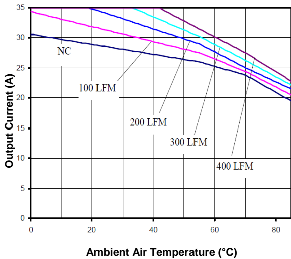
Figure 7. Derating Curve for Airflow Direction 1 (Ref. Figure. 8 for Airflow Direction; typical Vin, open frame, unit soldered onto a fixture board.)
