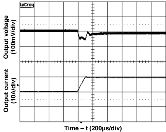
Figure 6. Transient Load Response (Typical Vin, 50% to 75% full load step at a slew rate 0.1A/µs)
