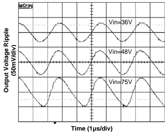
Figure 4. Output Ripple Voltage at Full Load
