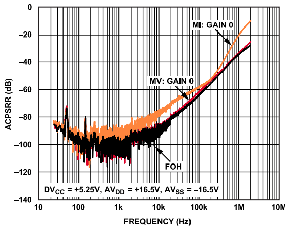
Figure 51. ACPSRR of HCAV_{DDx} vs. Frequency
