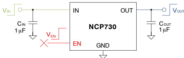
Figure 59. Circuit – Floating EN Pin
