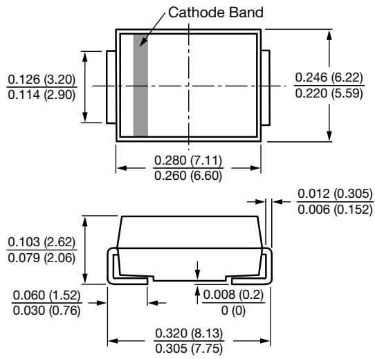
SMC (DO-214AB)
