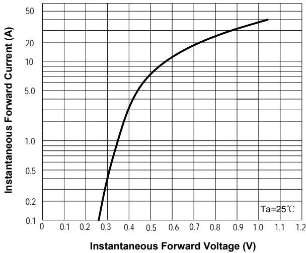
FIG3: Forward Voltage
