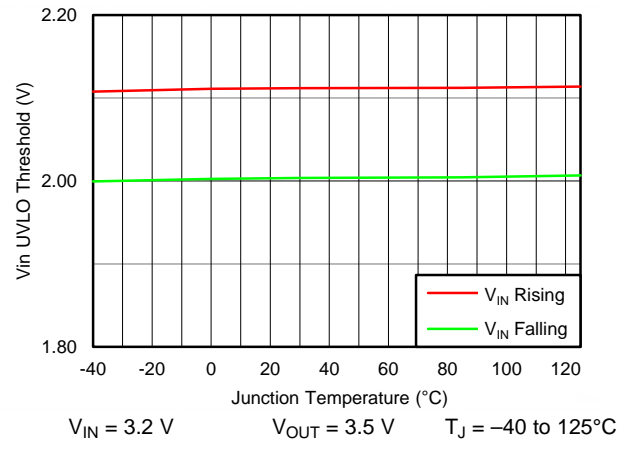
Figure 12. V_{IN} UVLO Threshold Rising/Falling vs Junction Temperature
