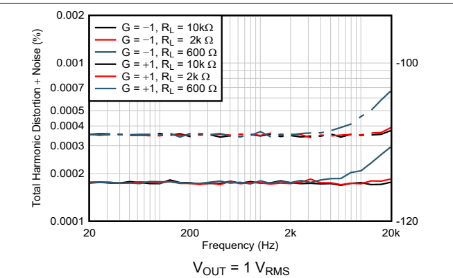
Figure 6-31. THD+N vs Frequency
