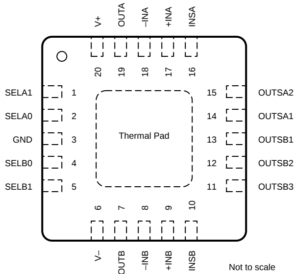
Figure 5-1. OPA3S328 RGR (20-Pin VQFN) Package, Top View
