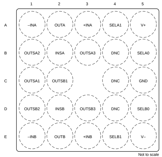
Figure 5-2. OPA3S328 YBJ (24-Pin DSBGA Preview) Package, Top View
