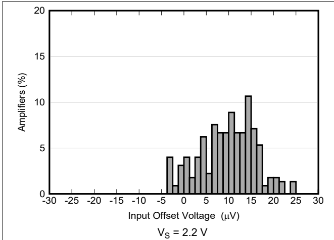
Figure 6-2. Offset Voltage Production Distribution
