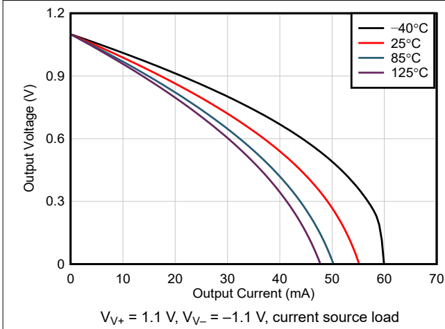
Figure 6-20. Output Voltage Swing vs Output Current
