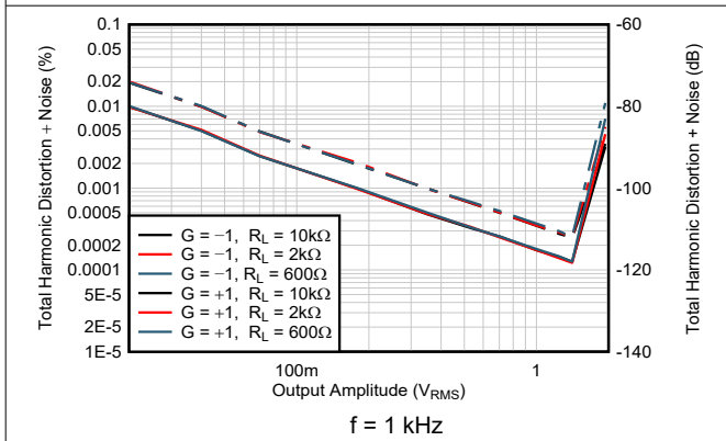
Figure 6-30. THD+N vs Amplitude
