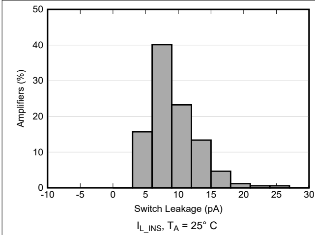
Figure 6-38. Switch Input Leakage Current Histogram
