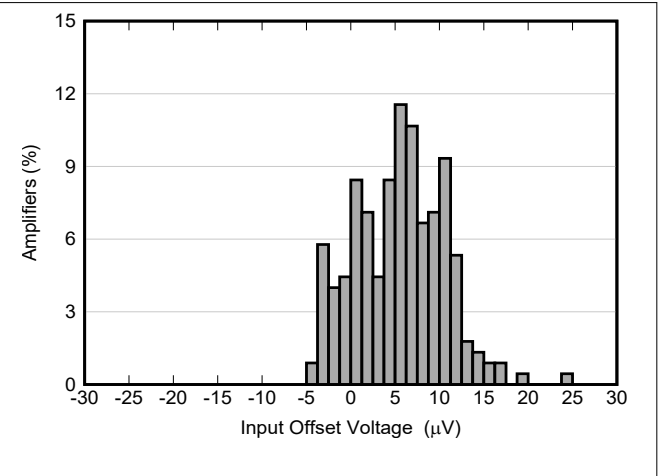
Figure 6-3. Offset Voltage Production Distribution
