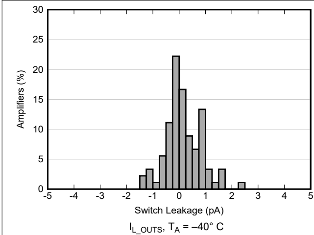
Figure 6-40. Switch Output Leakage Current Histogram
