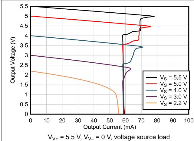
Figure 6-24. Output Voltage Swing vs Output Current
