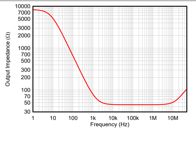
Figure 6-25. Open-Loop Output Impedance vs Frequency
