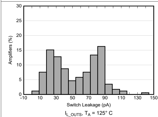
Figure 6-42. Switch Output Leakage Current Histogram
