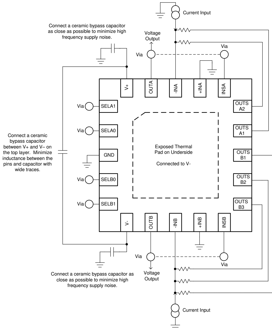
Figure 11-1. Layout Example
